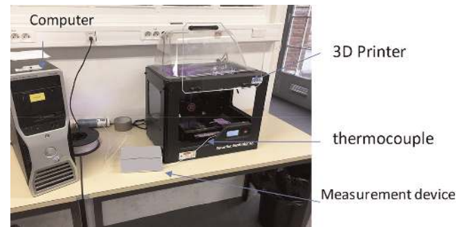
Fig. 3. System setup
