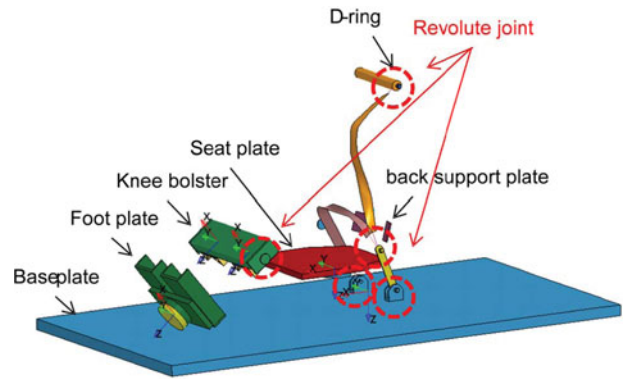
Fig. 1. Buck model.
