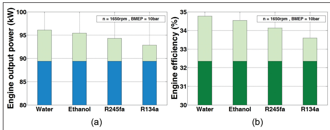
Figure 10. (a) Engine output power and (b) engine efficiency gain as functions of the working fluid. rpm: r/min; BMEP: brake mean effective pressure.
