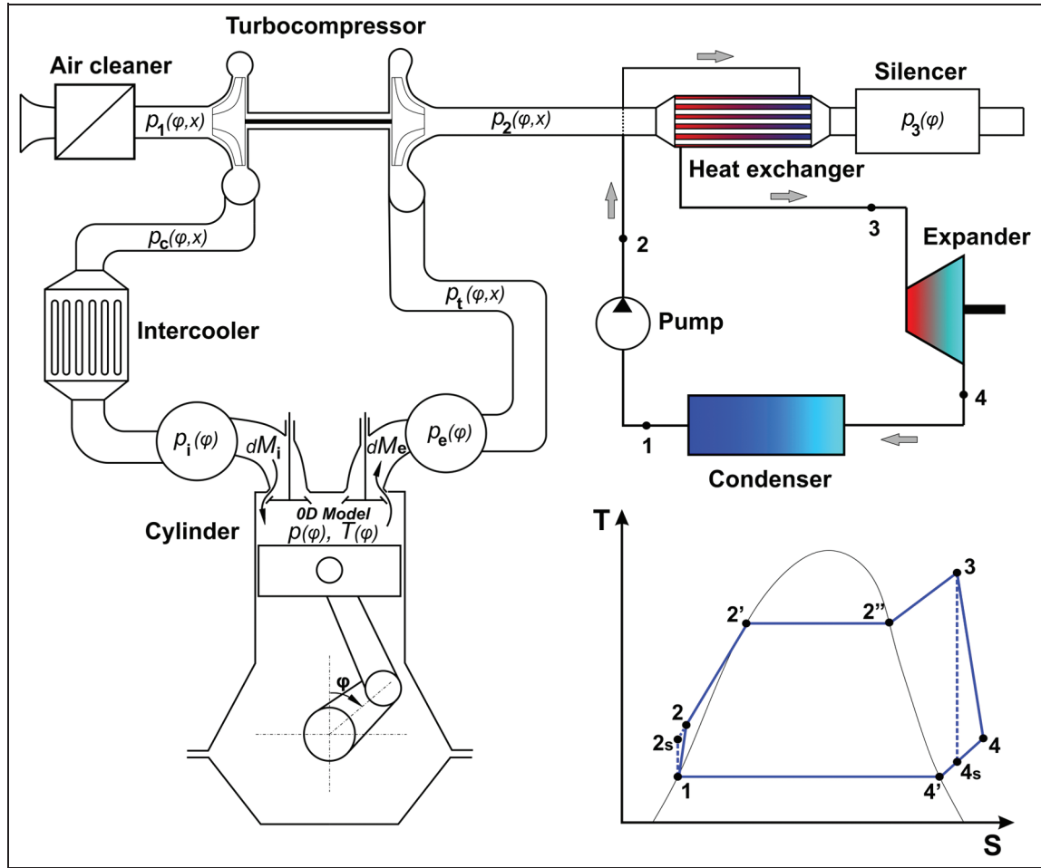
Figure 1. Models of the engine and the RC.
