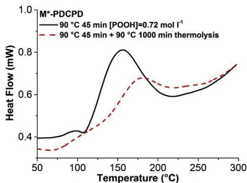
Fig. 3. DSC thermograms before (full line) and after 1000 min thermolysis at 90 °C (dashed line) for M*-PDCPD exposed 45 min at 90 °C under air.
