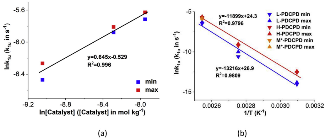
Fig. 13. Change of k_{1u} with catalyst concentration at 120 °C (a) and Arrhenius plot of k_{1u} for different PDCPD systems (b). (NB: min and max values refer to the possible uncertainties associated to the determination method of k_{1u} and are given in Table 2).
