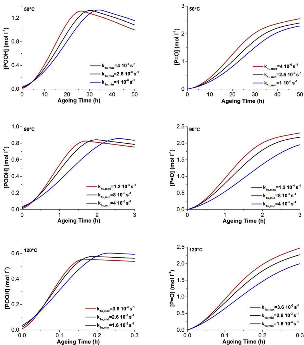
Fig. 14. Numerical simulations for thermolysis of POOH with different value of k_{1u} (and [POOH]_{t=0} values from Table 1).
