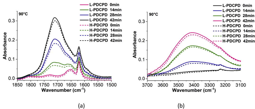
Fig. 7. FTIR spectra of L-PDCPD (full line, 13.3 \mu\text{m} thickness) and H-PDCPD (dashed line, 12.8 \mu\text{m} thickness) exposed at 90 °C under air.
