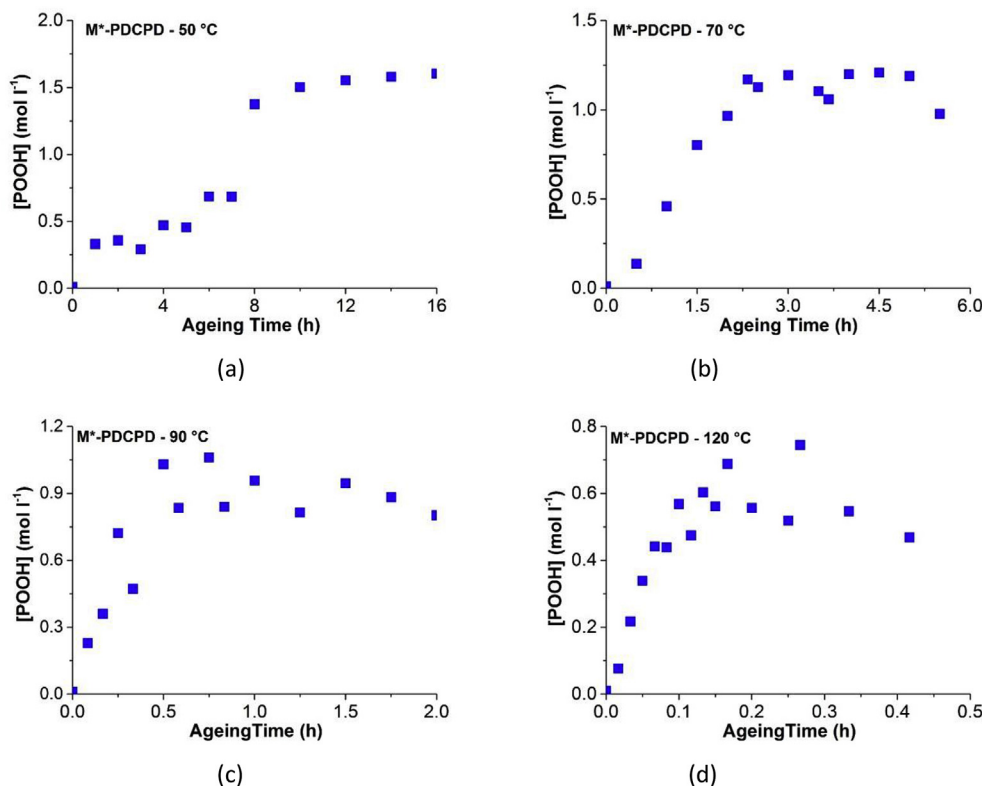
Fig. 2. Changes in hydroperoxides concentration for thermal oxidation in PDCPD medium* at 50 (a), 70 (b), 90 (c) and 120 °C (d).
