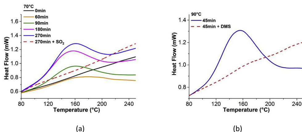
Fig. 1. DSC thermograms of M*-PDCPD exposed at 70 °C under air for various ageing times up to 270 min before (full line) and after (dashed line) SO 2 treatment (a), and exposed 45 min at 90 °C under air before (full line) and after (dashed line) DMS treatment (b).
