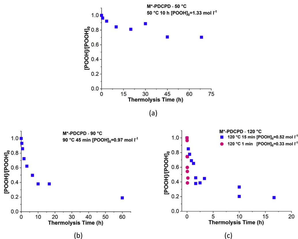
Fig. 4. Changes in normalized hydroperoxides concentration ( [\text{POOH}]_0 is the hydroperoxide concentration after ageing under air – see Fig. 2) for thermolysis of M*-PDCPD at 50 (a), 90 (b) and 120 °C (c). NB: time to totally destroy POOH at 50 °C was too long so that thermolysis were interrupted after 70 h.
