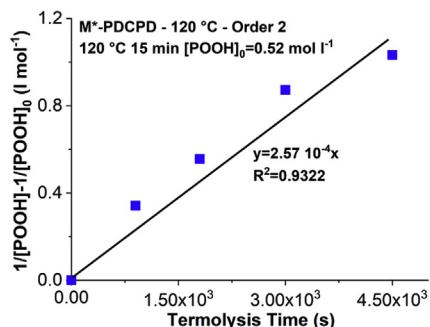
Fig. 9. Linear equation of order 1 (left) and 2 (right) for M*-PDCPD thermolysis at pseudo plateau at 50 (a), 90 (b) and 120 °C (c). NB: the caption indicates the time and temperature for ageing under air, and the corresponding POOH concentration after ageing and before thermolysis – see Fig. 2).
