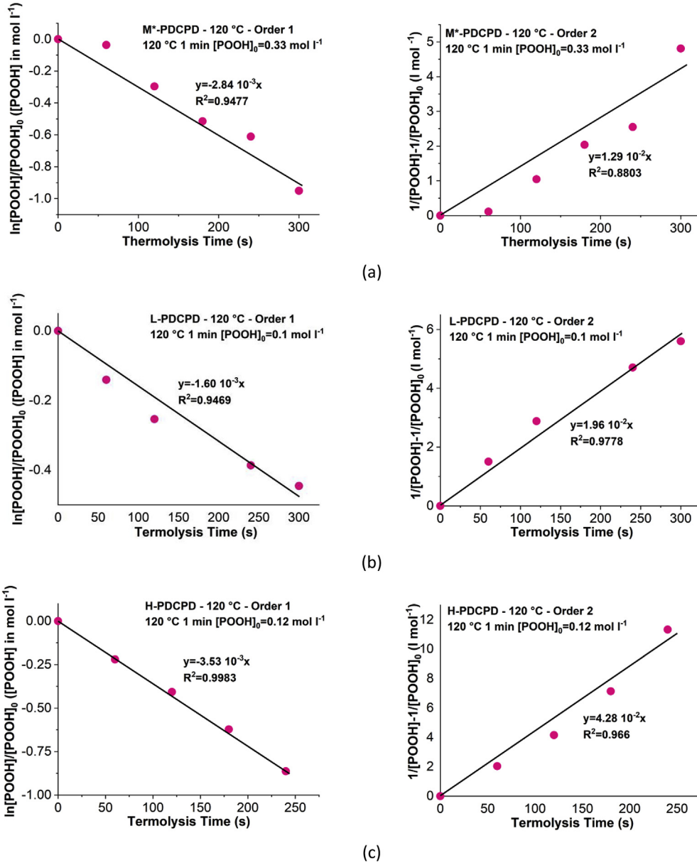
Fig. 11. Kinetic order 1 and 2 of thermolysis for M*-PDCPD samples aged 1 min at 120 °C (a); for L-PDCPD samples aged 1 min at 120 °C (b); for H-PDCPD samples aged 1 min at 120 °C (c). (NB: the caption indicates the ageing time and temperature under air, and the corresponding POOH concentration after ageing and before thermolysis – see Figs. 2 and 6).
