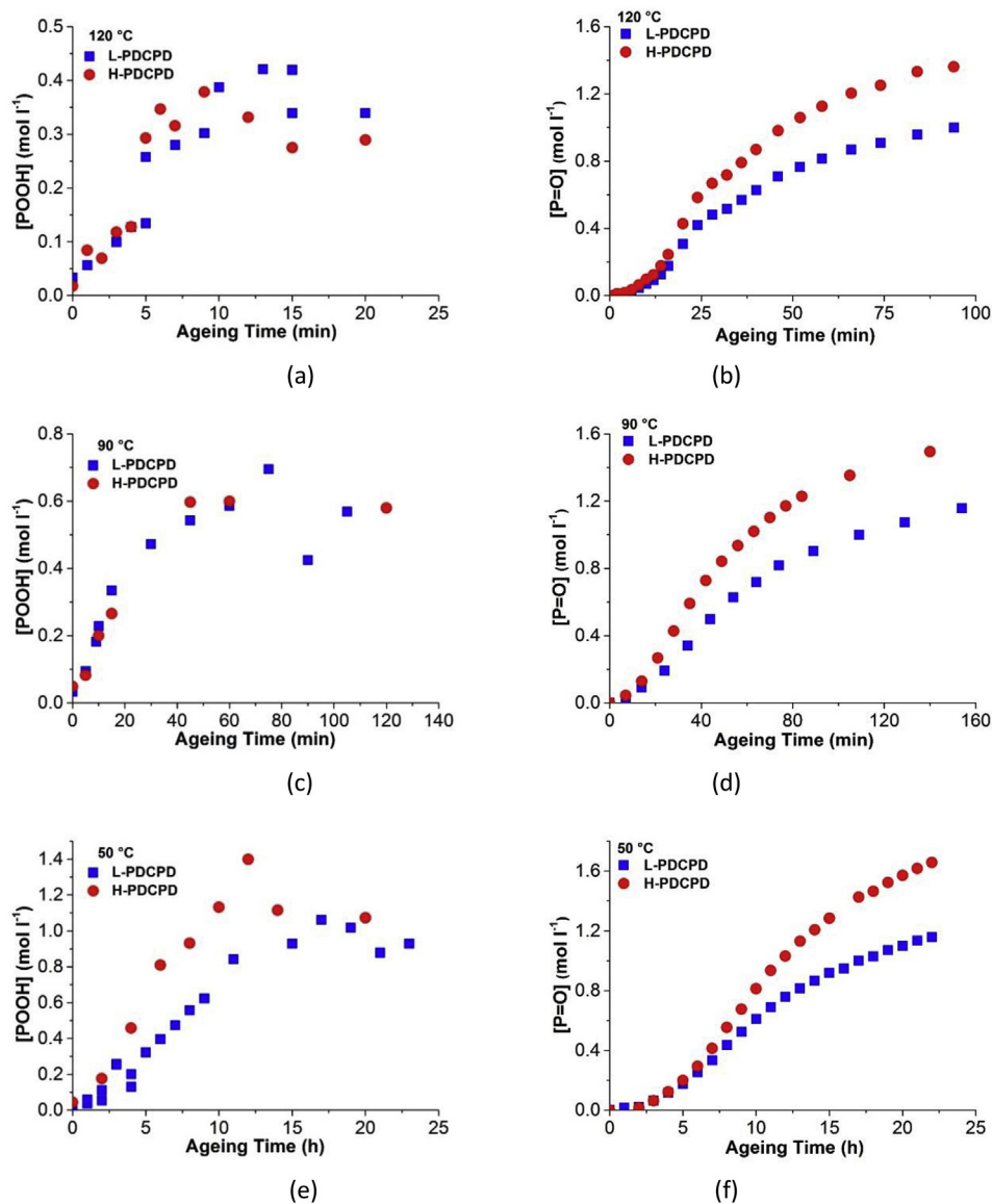
Fig. 6. Changes in hydroperoxides and carbonyls concentrations for L-PDCPD samples (■), or H-PDCPD samples (●) catalyst content thermally oxidized at 120, 90 and 50 °C under air.
