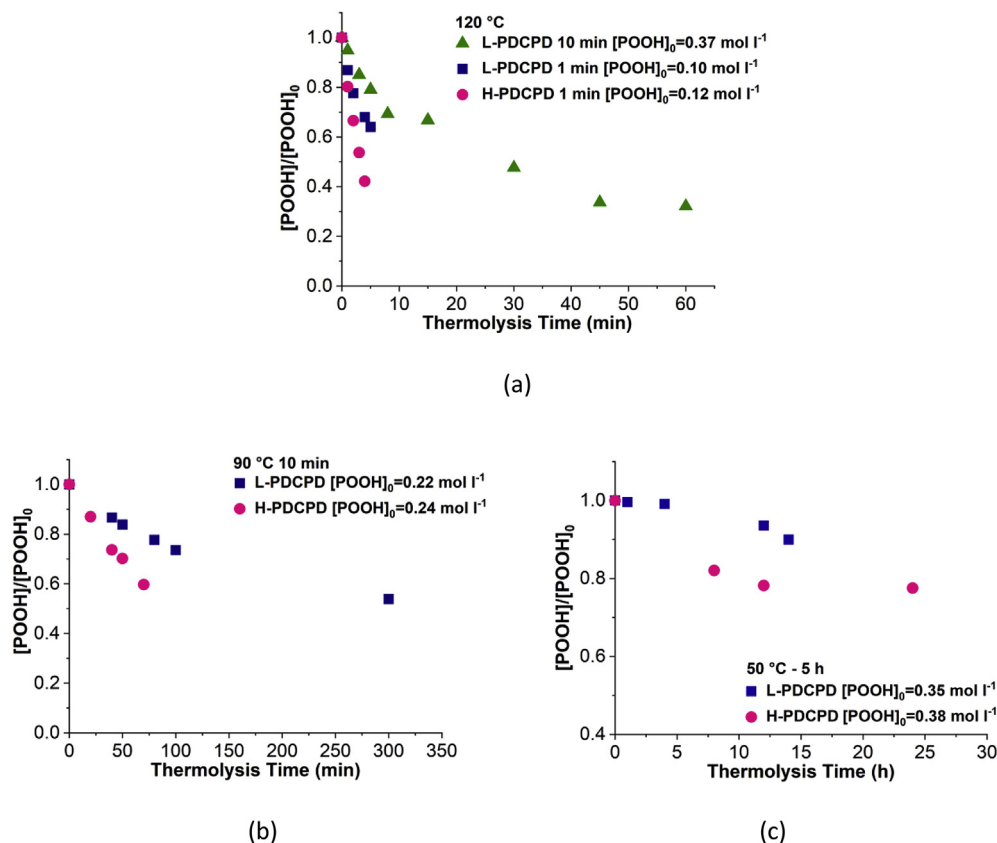
Fig. 8. Changes in hydroperoxides concentration for thermolysis of L-PDCPD (▲ or ■) and H-PDCPD (●) at 120 (a), 90 (b) and 50 °C (c). NB: the caption indicates the temperature and time for ageing under air, and the corresponding POOH concentration after ageing and before thermolysis – see Fig. 6.
