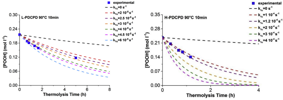
Fig. 12. Numerical simulations for thermolysis of POOH (Eq. (13)) with different value of k_{1u} at 90 °C. NB: the dashed line with k_{1u} = 0 corresponds to the contribution of k_{1b} in thermolysis at initially low POOH concentration.
