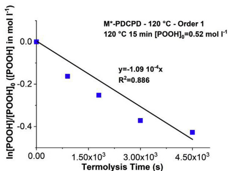
Fig. 9. Linear equation of order 1 (left) and 2 (right) for M*-PDCPD thermolysis at pseudo plateau at 50 (a), 90 (b) and 120 °C (c). NB: the caption indicates the time and temperature for ageing under air, and the corresponding POOH concentration after ageing and before thermolysis – see Fig. 2).
