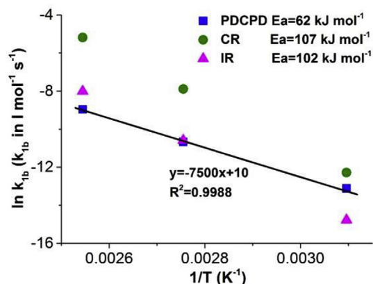
Fig. 10. Arrhenius plot of k_{1b} values coming from thermolysis for PDCPD (■), CR (●) [24], IR (▲) [17] from best fitting of oxidation curves.
