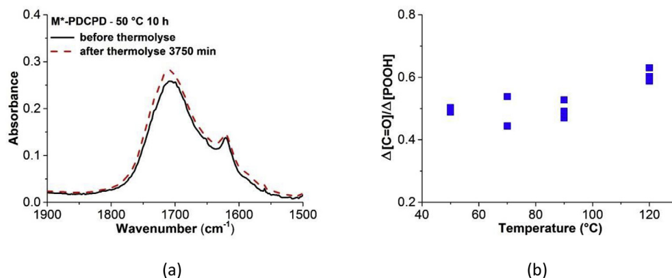
Fig. 5. FTIR spectra for PDCPD before (full line) and after (dashed line) thermolysis at 50 °C (a) and apparent carbonyl yield as a function of temperature (b).
