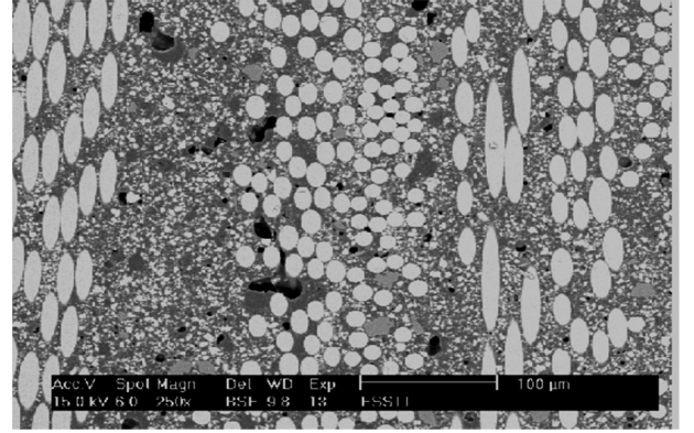
Fig. 2. Microstructure of SMC composite: Bundle of fibers.
