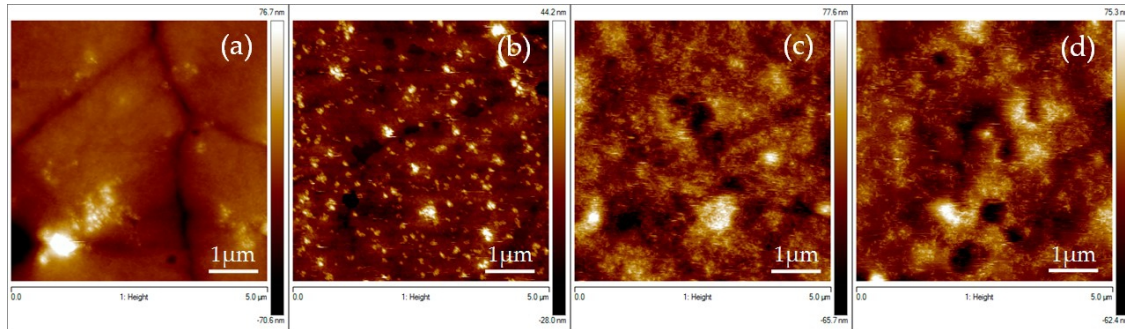
Figure 5. 5 \times 5 \mu\text{m} AFM micrographs showing the morphology of the composite PVDF thin film on silicon substrate with different concentrations of NPs (a) 0.5 wt % of non-functionalized NPs; (b) 0.5 wt % of functionalized NPs; (c) 1 wt % of non-functionalized NPs; and (d) 1 wt % of functionalized NPs.
