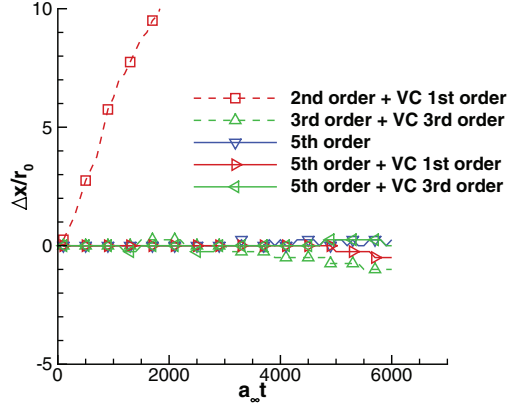
(c) x trajectory error, medium
