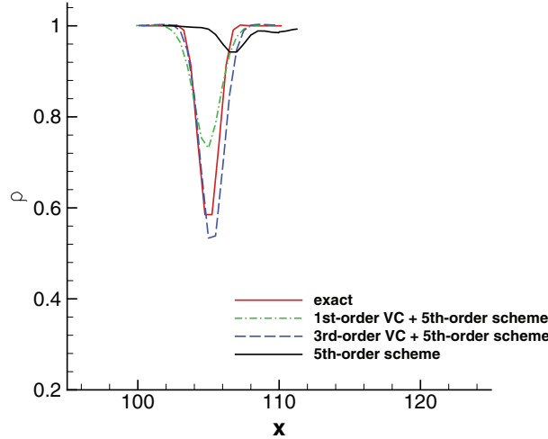
(c) coarse, \varepsilon = 0.04, \varepsilon/\mu = 1.67
