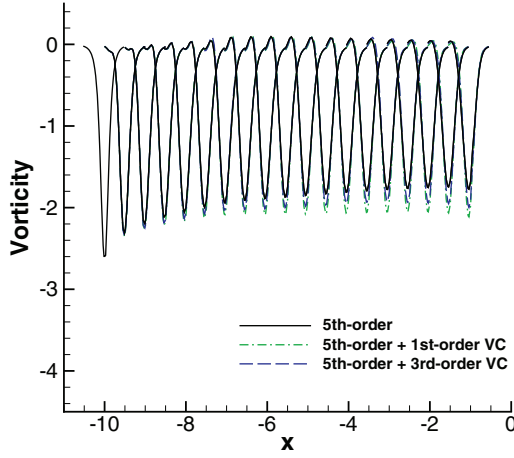
(a) coarse mesh
