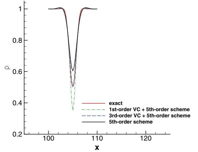
(b) medium, \varepsilon = 0.02, \varepsilon/\mu = 1.67
