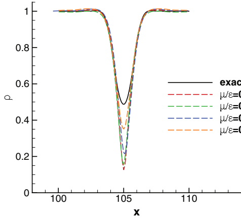
(a) 1st-order confinement
