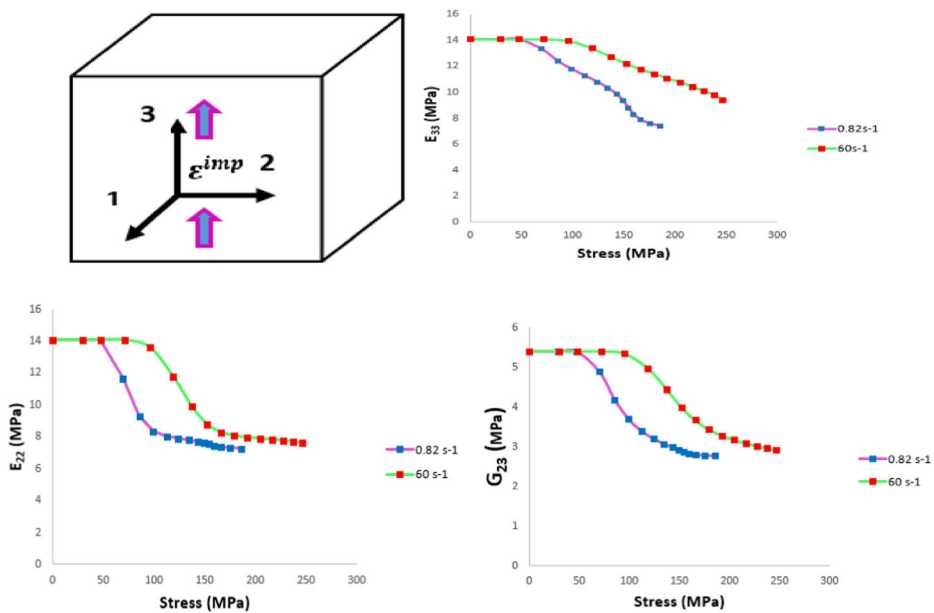
Fig. 8 Predicted stiffness reduction (E33, E22 and G23) at three strain rates (0.82 and 60 s -1 )
