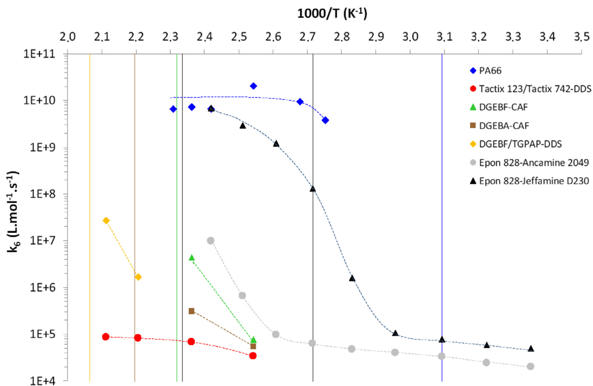
Fig. 9. Arrhenius graphs between 25 and 250°C of the rate constant k_g for the six EPO-DA networks under study and aliphatic polyamides. The vertical solid straight-lines indicate the position of the T_g of the different materials.
