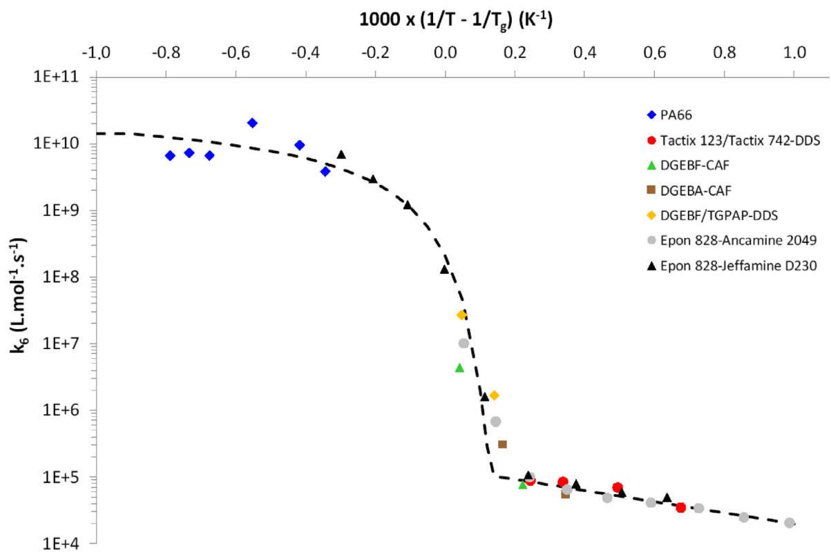
Fig. 10. Master curve around the glass transition temperature for the rate constant k_g of EPO-DA networks and aliphatic polyamides. Modeling of the impact of the thermodynamic transition with Eq. (18).
