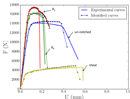
Fig. 5. Comparison between numerical and experimental force versus displacement curves for a temperature of 25^\circ\text{C} and a strain rate of 1 \text{ s}^{-1} .
