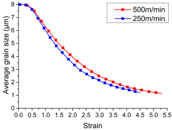
Fig. 17. Evolution of average grain size with increasing strain.
