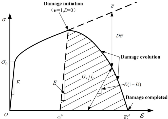
Fig. 4. Stress-strain curve of material damage degradation.
