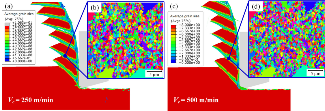
Fig. 12. Average grain size distribution simulated by FE (a and c) and the grain morphology simulated by CA method (b and d) at cutting speed of 250 m/min (a and b) and 500 m/min (c and d).
