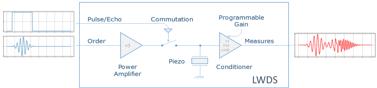
Figure 1 : High frequency commutation with LWDS
