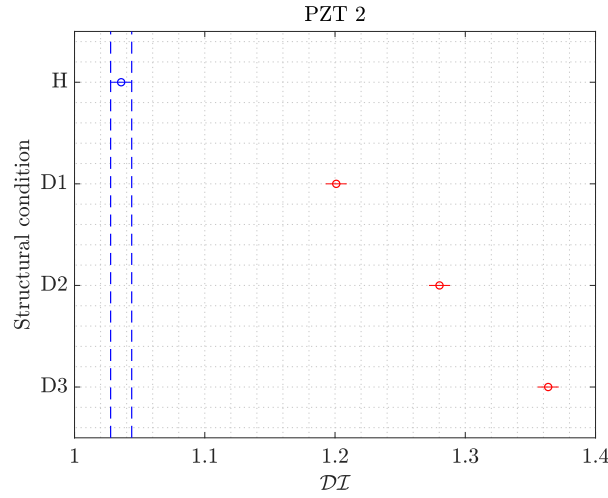
Figure 7: Classification of the clusters of different damage' states using ANOVA of \mathcal{DI} . 3 groups (in red) have means significantly different from healthy H .
