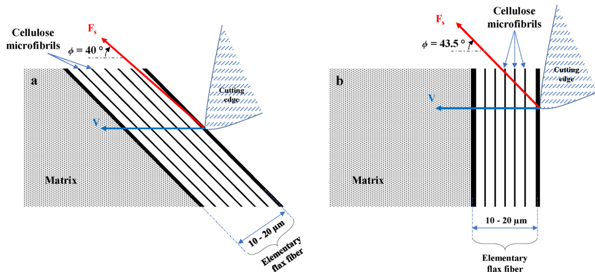
Fig. 10. Schematic illustration of the microscopic contact between the cutting tool edge and the flax fiber. a) at \theta = 45^\circ and b) at \theta = 90^\circ .
