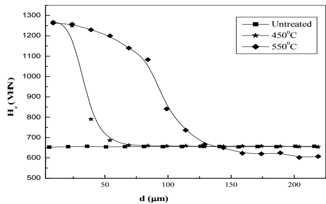
Fig.1 Microhardness vs. depth profiles of samples treated at 450 °C and 550 °C for 6 h. Plasma nitriding at lower as well as elevated temperatures raises the hardness of CrMoV steel significantly. Hardness achieved in the present study is much higher than the previously reported hardness values [13-15]. Hardness values achieved by elevated temperature plasma nitriding of CrMoV steel by other workers are shown in the following Table 1.
