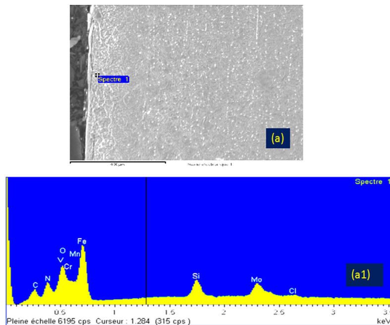
Fig.3 SEM and EDS (a-a1) of CrMoV steel after plasma nitriding at 450^\circ\text{C} for 6h.
