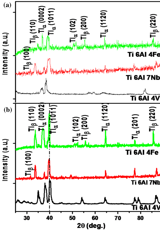
Fig. 2 XRD patterns of milled titanium powders alloys versus: a) 2-h and b) 18-h milling
