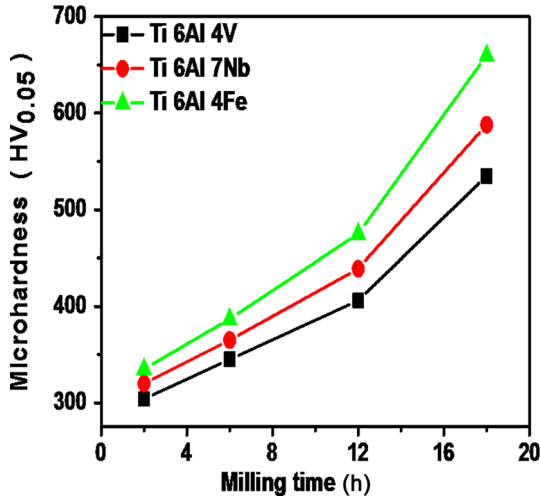
Fig. 5 Vickers hardness values of titanium alloys versus milling time
