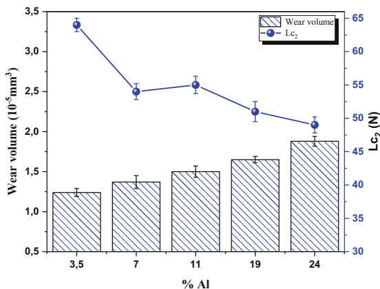
Fig. 4. Critical load and wear volume of CrAlN coatings under different Al content
