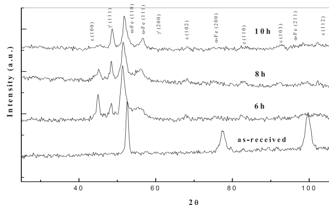
Fig. 2. Bragg-Brentano mode of X-ray diffraction of as-received and samples after plasma nitriding for variable times.
