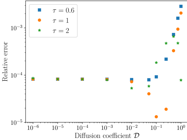
FIG. 4. Relative errors of the diffusion coefficient.
