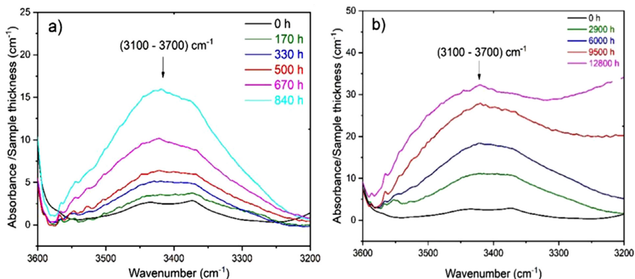
Fig. 4. Changes in the hydroxyl region of the FTIR spectrum of Si-XLPE before and after radio-thermal ageing in air under 400 Gy.h -1 at 21°C (a) and under 8.5 Gy.h -1 at 47°C (b).
