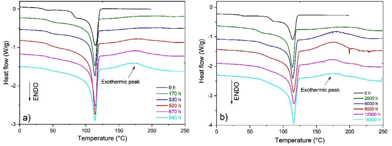
Fig. 5. Changes in the DSC thermogram of Si-XLPE before and after radio-thermal ageing in air under 400 Gy.h -1 at 21°C (a) and under 8.5 Gy.h -1 at 47°C (b).
