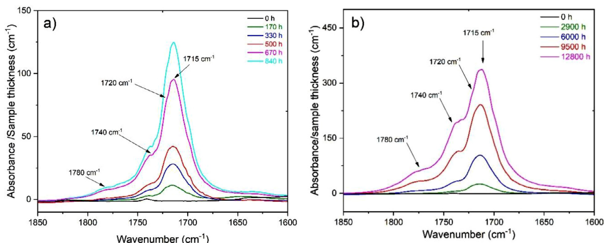
Fig. 3. Changes in carbonyl region of the FTIR spectrum of Si-XLPE before and after radio-thermal ageing in air under 400 Gy.h -1 at 21°C (a) and under 8.5 Gy.h -1 at 47°C (b).
