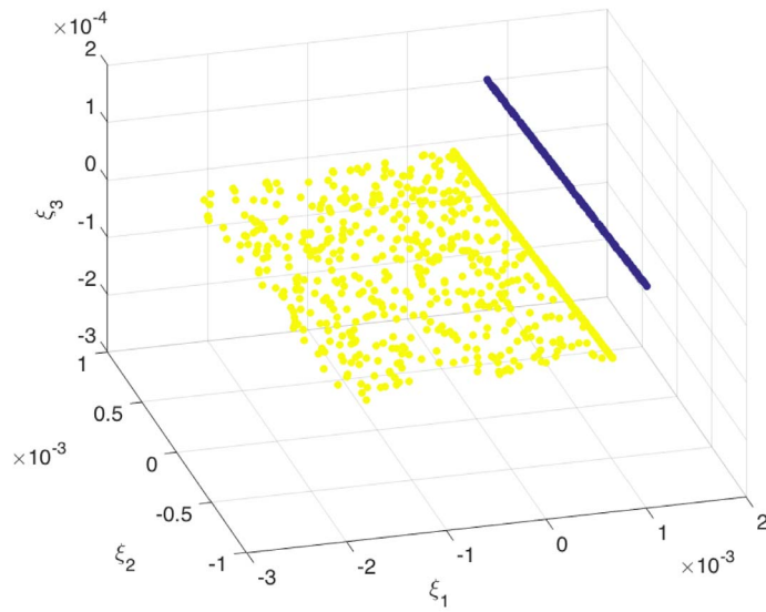
Figure 26. Slow manifold related to elastic–plastic behavior operating within the elastic domain and on the elastic domain boundary colored according to the tangent modulus.
