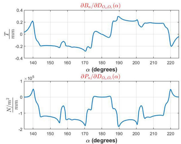
Fig. 18 Sensitivity of B_n and P_n for small changes in D_{O_s, O_r} . Operating point: \gamma = 0 degrees, I_p = 0.5 A, \tau = \pi/2 rad, \rho = 0
