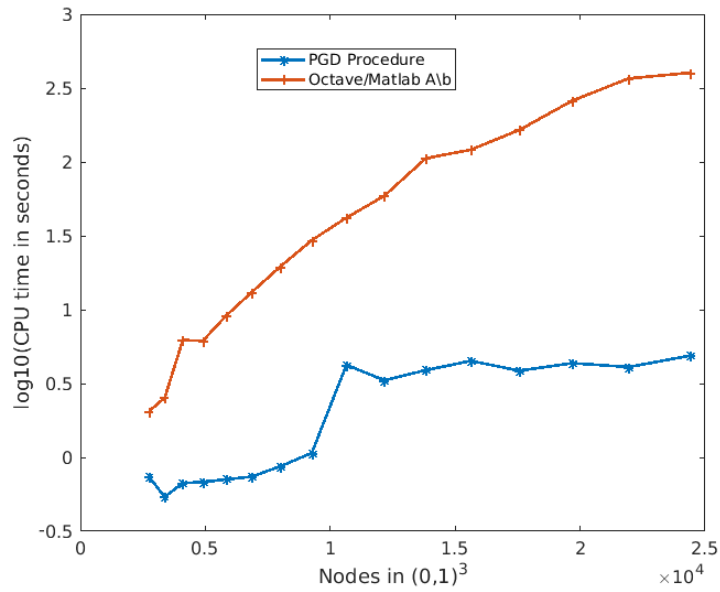
Figure 10. Comparison made in [37] in terms of CPU time between the PGD method and the traditional \backslash b Matlab-Octave method for the resolution of the Poisson equation as a function of the number of nodes in the discretization of the equation.
