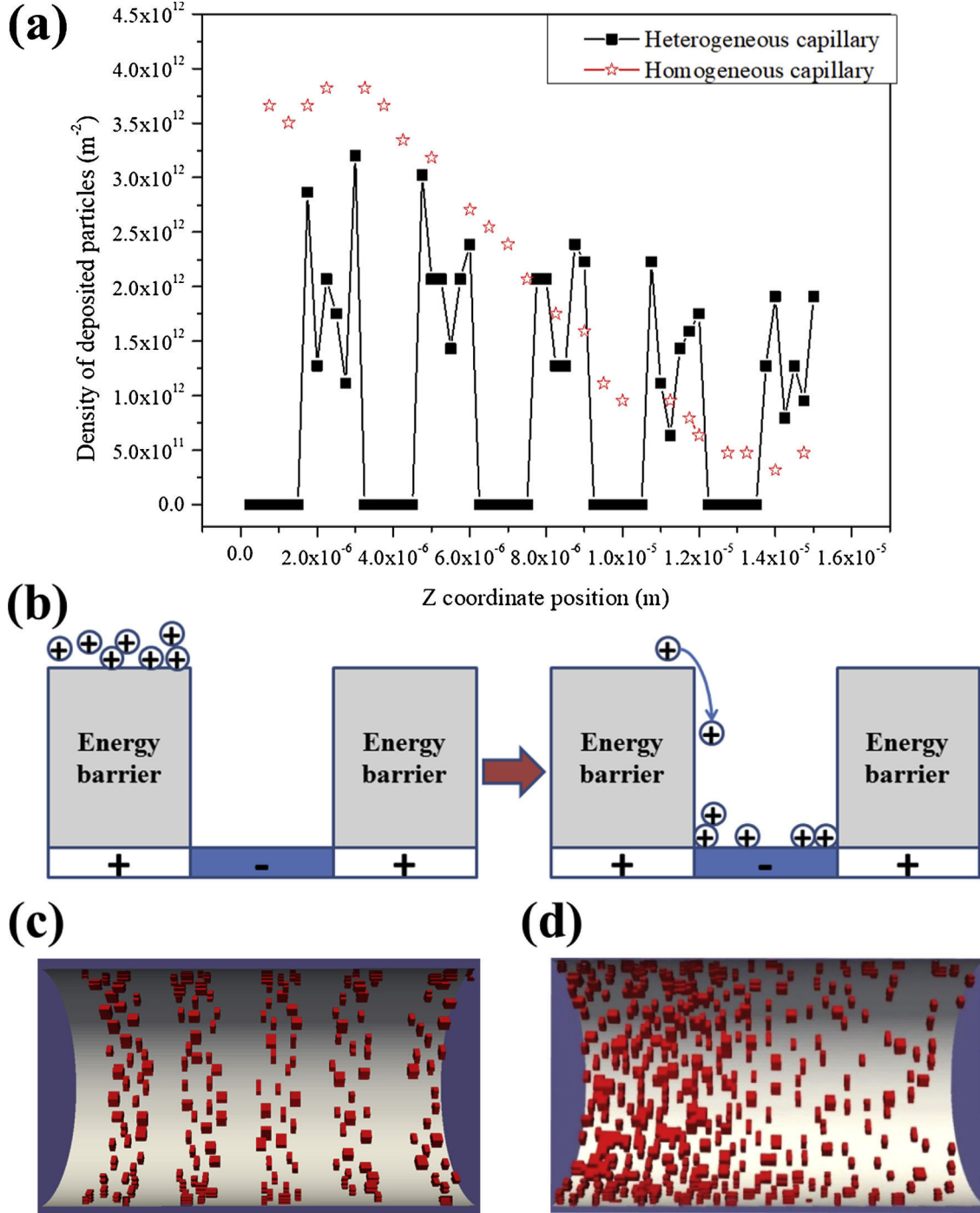
Fig. 3. (a) Spatial density distribution of the deposited particles versus the z coordinate at N = 2000 , Pe = 1.5 \times 10^{-3} for both heterogeneous ( \lambda = 5 and \theta = 0.5 ) and homogeneous capillary; (b) schematic representation of particle behavior near the boundaries between the favorable and unfavorable strips (after Nazemifard et al. [32,41]). 3D sectional view of the heterogeneous (c) and homogeneous (d) capillary. The red objects represent the deposited particles; the flow occurs from left to right. (For interpretation of the references to colour in this figure legend, the reader is referred to the web version of this article.)
