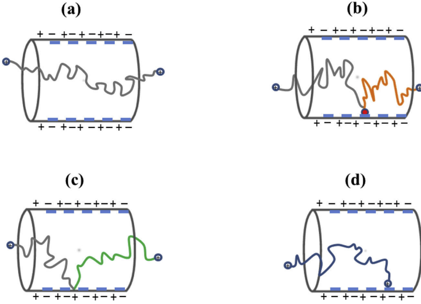
Fig. 2. Sketches of possible particle trajectories: (a) flowing through the capillary without deposition; (b) particle approaching a deposited particle (in grey line) and bouncing back to the bulk flow (in orange line); (c) particle approaching a repulsive zone and bouncing back to the bulk flow (in green line); (d) particle approaching an attractive zone and deposited when enough surface is available. (For interpretation of the references to colour in this figure legend, the reader is referred to the web version of this article.)
