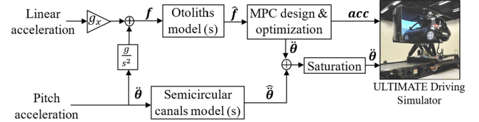
Fig. 1. Control design for the DS's movement restitution based MPC along the x -axis.
