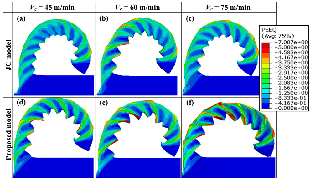
Fig. 16 Numerical chip morphology predicted with the JC (a–c) and the proposed rheological models for different cutting speeds ( f = 0.15 \text{ mm/rev} ) (d–f)
