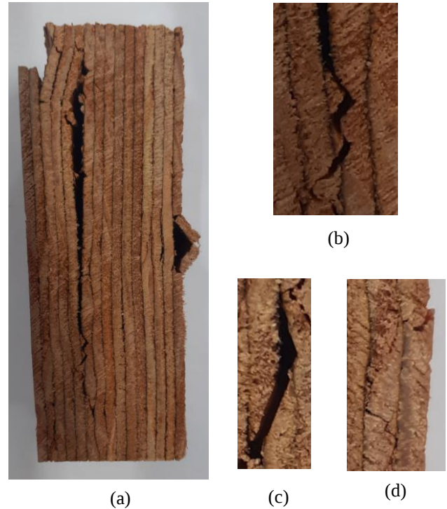
Figure 6: (a) Edgewise perpendicular to the grain compression specimen failure, (b) sawtooth propagation, (c) inter-plies growth ring limit propagation (c), inter-plies lathe check propagation (d)
