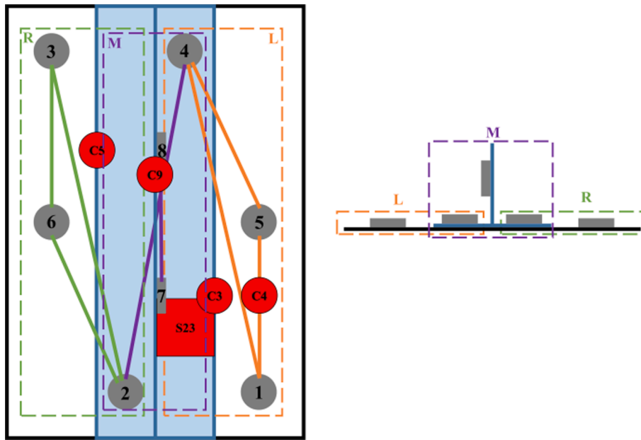
Fig. 7. Sensor path selection for stiffness degradation assessment. The panel is partitioned into left (L), middle (M) and right (R) sections with dash lines, as seen from the skin (DIC) side. The sensor paths within each section are plotted with the corresponding colour of the section.
