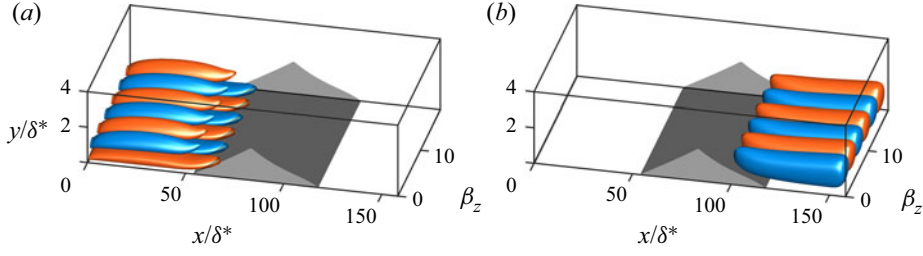
Figure 21. Optimal resolvent mode at \beta = 2 and St_L = 10^{-4} , real part of w of the forcing (a) and real part of u of the response (b). Isosurfaces at 20 % and -20 % of the maximum absolute value are plotted.
