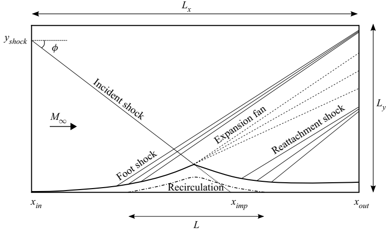
Figure 1. Sketch of the numerical domain and typical structure of the oblique shock wave/boundary layer (OSWBLI).
