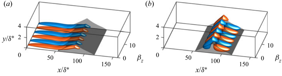
Figure 19. Optimal resolvent mode at \beta = 0.25 and St_L = 10^{-4} , real part of w . Iso-surfaces at 40 % and -40 % of the maximum absolute value are plotted in red and blue. The dark grey surface is the recirculation bubble of the base flow (homogeneous in z ).
