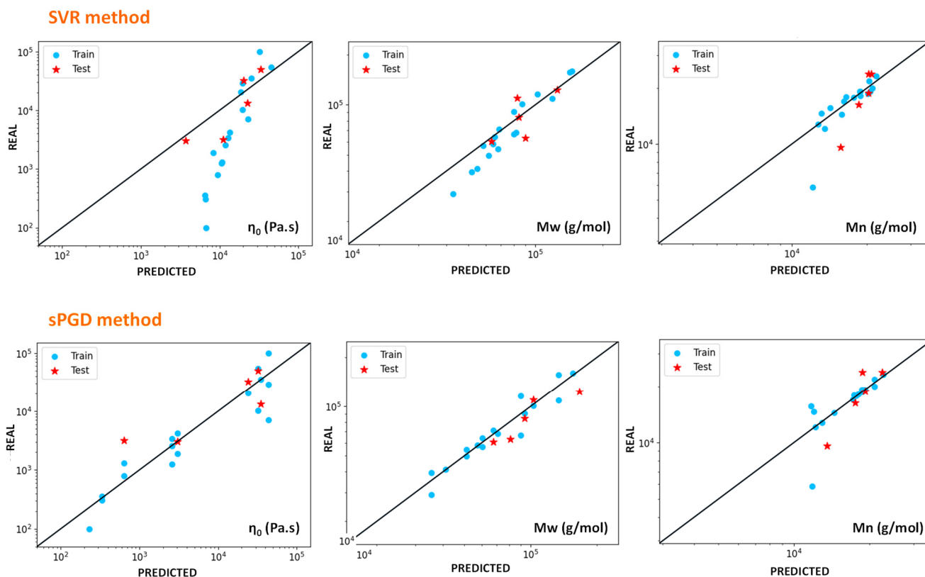
Figure 12. Results of zero-shear viscosity and weight and number average molecular weights predicted by SVR and sPGD methods versus the experimental ones. The blue dots correspond to training data, and the red stars correspond to test data for HDPE and UHMWPE indiscriminately.
