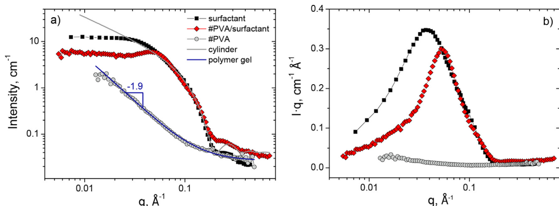
Fig. 2. The scattering curves in I(q) (a) and I \cdot q (b) coordinates for #PVA/potassium oleate/C 8 TAB system cross-linked with borate (red diamonds) and its components: potassium oleate/C 8 TAB solution (black squares) and #PVA (grey circles) in D 2 O. Concentrations: 4 wt% PVA, 2.5 wt% potassium oleate, 0.8 wt% C 8 TAB, 0.018 M potassium borate (molar fraction of borate with respect to PVA repeat units – 0.02). Grey line is a fit of the scattering curves by a form-factor of cylinder with radius R = 18.6 \pm 0.2 Å. Blue line is a fit of the scattering curve by a generalized Ornstein-Zernike (gel) model with mesh size \xi = 26 nm and fractal dimension D = 2.06 .
