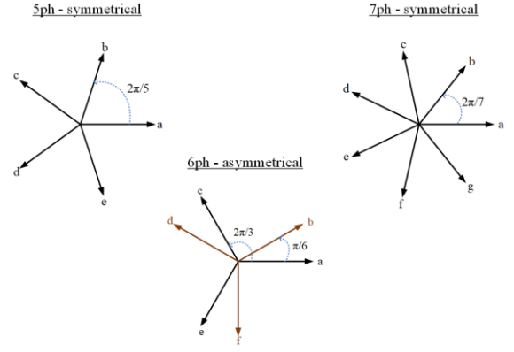
Fig. 2. Electrical angle shift between motor phase among studied topologies
