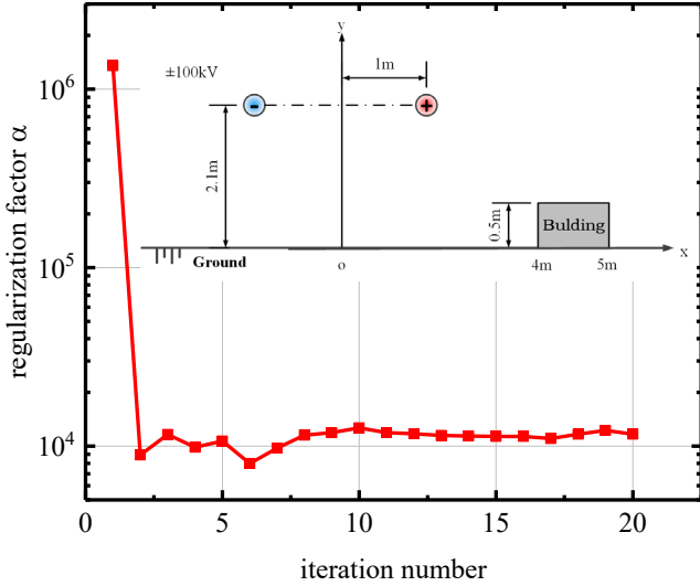
Fig. 9. the regularization factor \alpha determined by the formula (33) during the iterations.
