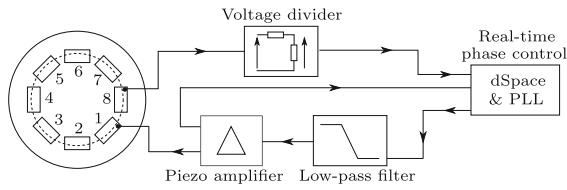
Fig. 3 Experimental setup for the symmetric mode (0, 1) measurement
