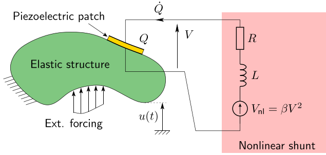
Figure 1. Nonlinear shunt principle.
