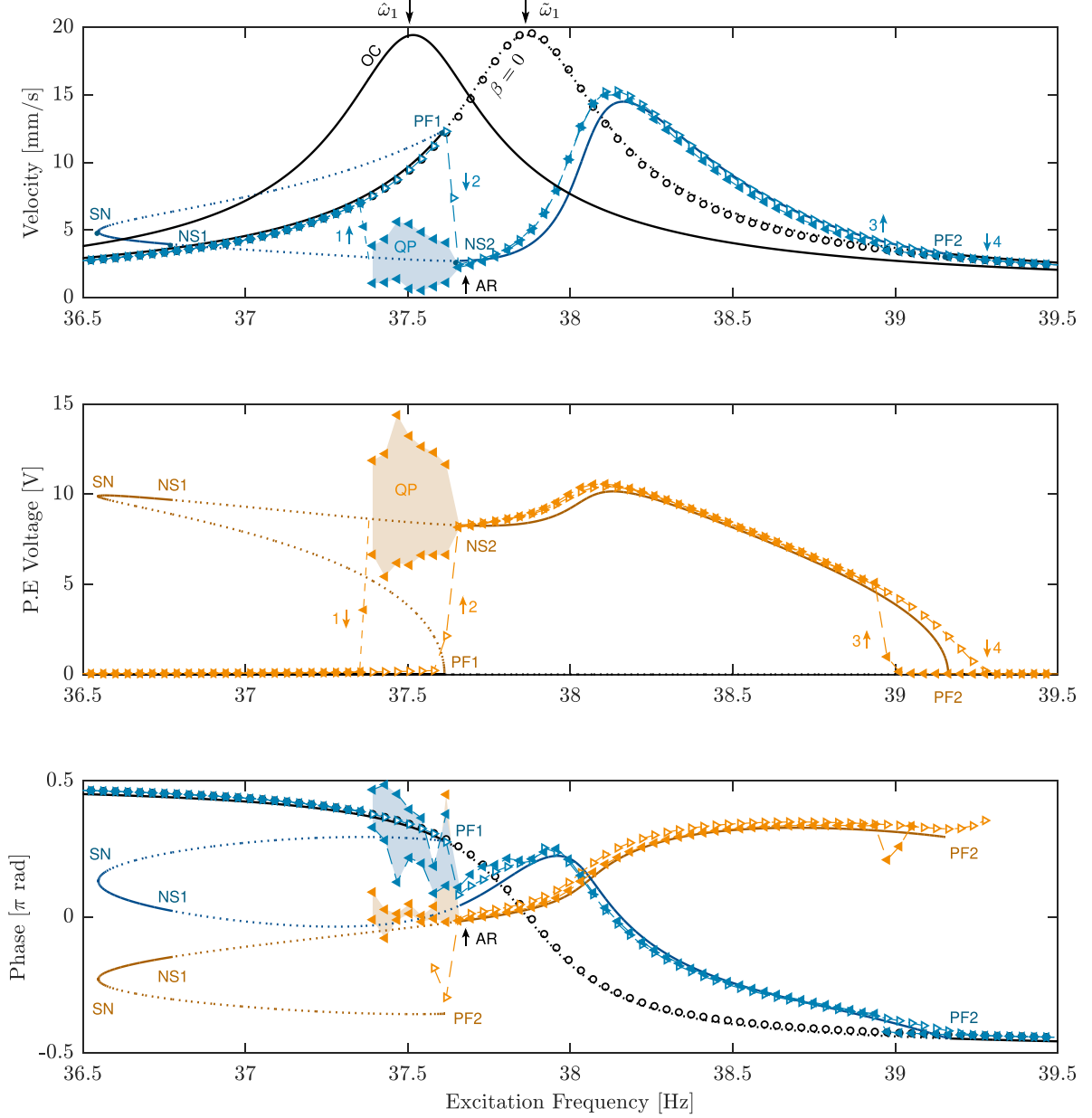
Figure 10. Experimental and numerical results comparison of the amplitudes of v_{H1} and V_{H1/2} and the phase angles \phi_v and \phi_V , plotted in blue and orange, respectively. The results are estimated with F = 0.45 mN, \xi_e = 0.002 , \xi_1 = 0.005 , \beta = 0.035 , and r_1 = 0.537 . The numerical data are shown in solid and dotted lines for stable and unstable solutions, respectively, in dark blue and orange, with the uncoupled solution plotted in black. The experimental data are plotted respectively with -\triangleright- and -\triangleleft- for sweeping up and down in the excitation frequency \Omega . The experimental uncoupled results are shown in -\circ- . The experimental and numerical quasi-periodic regime are shown in the shaded region and the dashed-dotted line, respectively.
