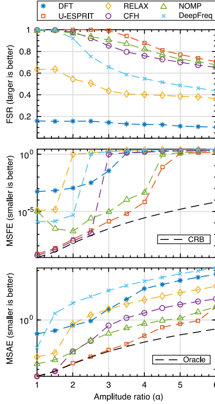
Fig. 12. Simulation results for varying amplitude magnitude scaling parameter \alpha . The signal length N = 2^7 , SNR = 40 dB, and model order P = 5 are pre-determined. The legend shown above applies to all plots, with sub-legends within the plots applying only to sub-plots.
