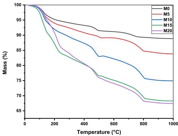
Fig. 13. Typical TGA curves collected at a heating rate of 10^{\circ}\text{C min}^{-1} for the various PCM mortars studied.
