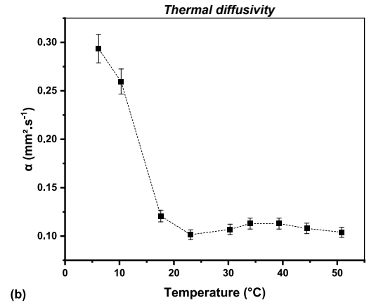
Fig. 10. Evolution curves of the (a) thermal conductivity and (b) thermal diffusivity obtained for the mPCM particles as a function of temperature.
