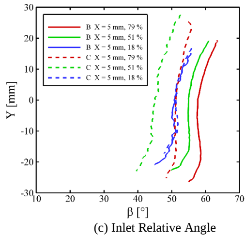
FIGURE 7: MEAN PROFILES AT NOMINAL OPERATING POINT IN BASE (B) AND CONTROLLED (C) CONFIGURATIONS AT X/C_X = 0.09
