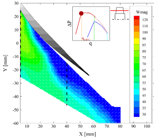
(b) PIV Plane at 51% of Blade Height
