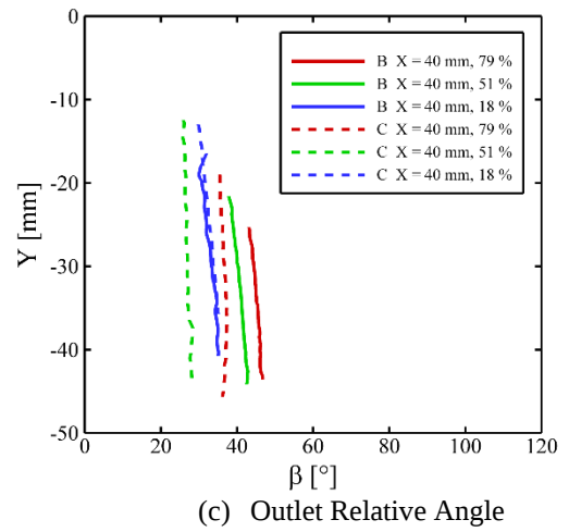
FIGURE 8: OUTLET AT NOMINAL OPERATING POINT IN BASE (B) AND CONTROLLED CONFIGURATIONS (C) X/C_X = 0.73
