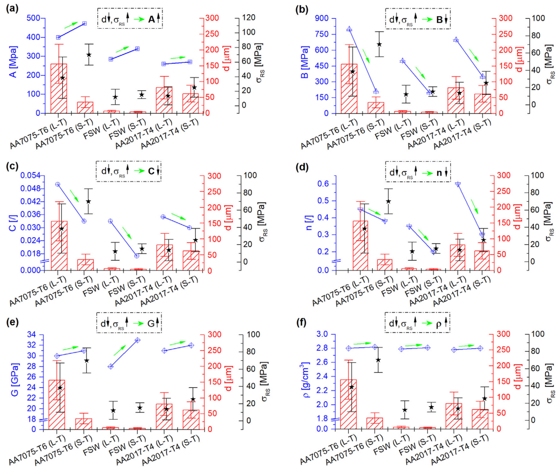
Fig. 14. Correlation between grain size, residual stress and material model parameters in specific regions and planes of dissimilar FSW 7075–2017 joint; (a) initial yield strength A , (b) strain hardening modulus B , (c) strain rate sensitivity C , (d) strain hardening exponent n , (e) shear modulus G and (f) density \rho .
