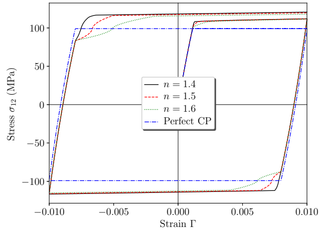
Fig. 11. Effects of the defect energy index n for constant higher-order dissipative parameters ( l_{en}/h = 1 , l_d/h = 0.25 , S_{\xi 0} = 10 MPa, H_{\xi} = 100 MPa).
