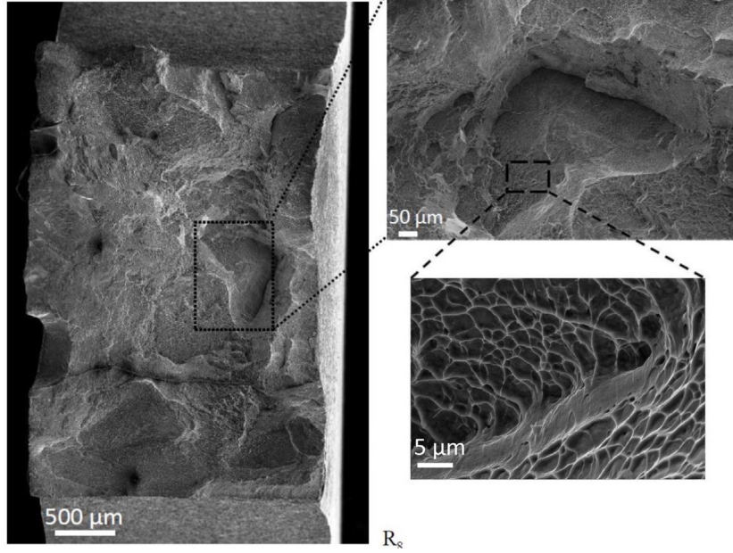
Fig. 3. SEM observations of the as-received \alpha + \beta Ti17 titanium alloy deformed at a strain rate of 0.1 \text{ s}^{-1} , a temperature of 25 \text{ }^{\circ}\text{C} showing the ductile aspect of fracture.
