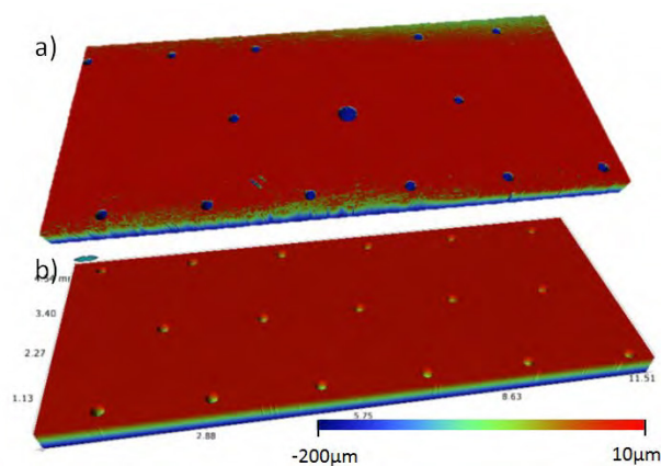
Fig. 5. Surface topography of the surface specimen a) face I containing 13 defects \varnothing 200\mu\text{m} and one defect \varnothing 400\mu\text{m} , b) face II containing 17 defects \varnothing 200\mu\text{m}
