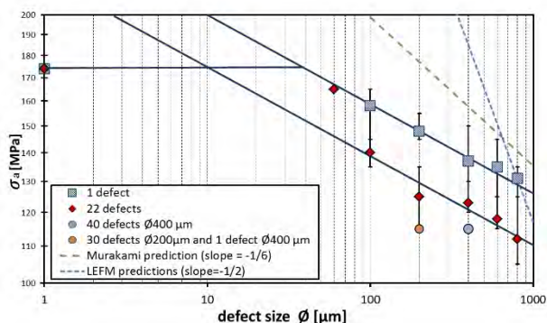
Fig. 6. Kitagawa-Takahashi diagram, AA7050alloy: experimental results for different defect size and number.
