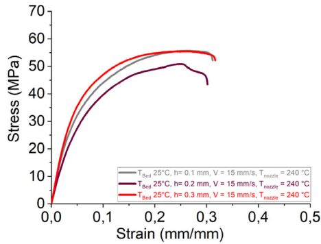
FIGURE 16 Tensile behavior of the printed specimens with the various layer height
