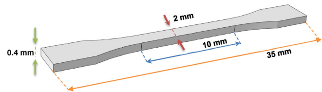
FIGURE 3 The geometry of the used specimen
