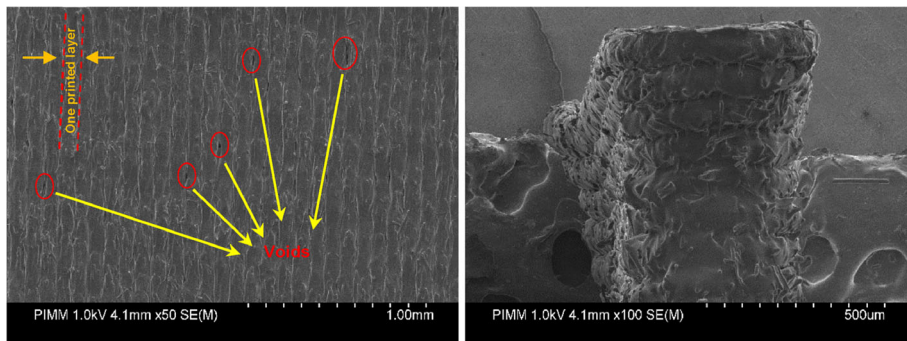
FIGURE 14 Scanning electron micrographs (SEM) related to the printed specimens at V = 13 mm/s
