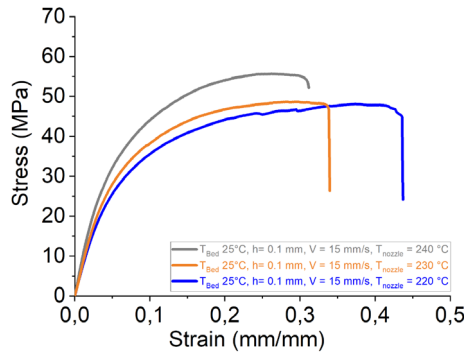
FIGURE 10 Tensile behavior of printed specimens under the various liquefier temperatures
