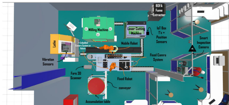
Fig. 7. ENSAM industrial platform 4.0, 3D-model.
