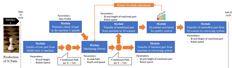
Fig. 8. Production plan example for a chess pawn.
