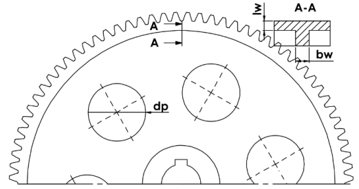
Fig. 4 The three design parameters added in Level II
