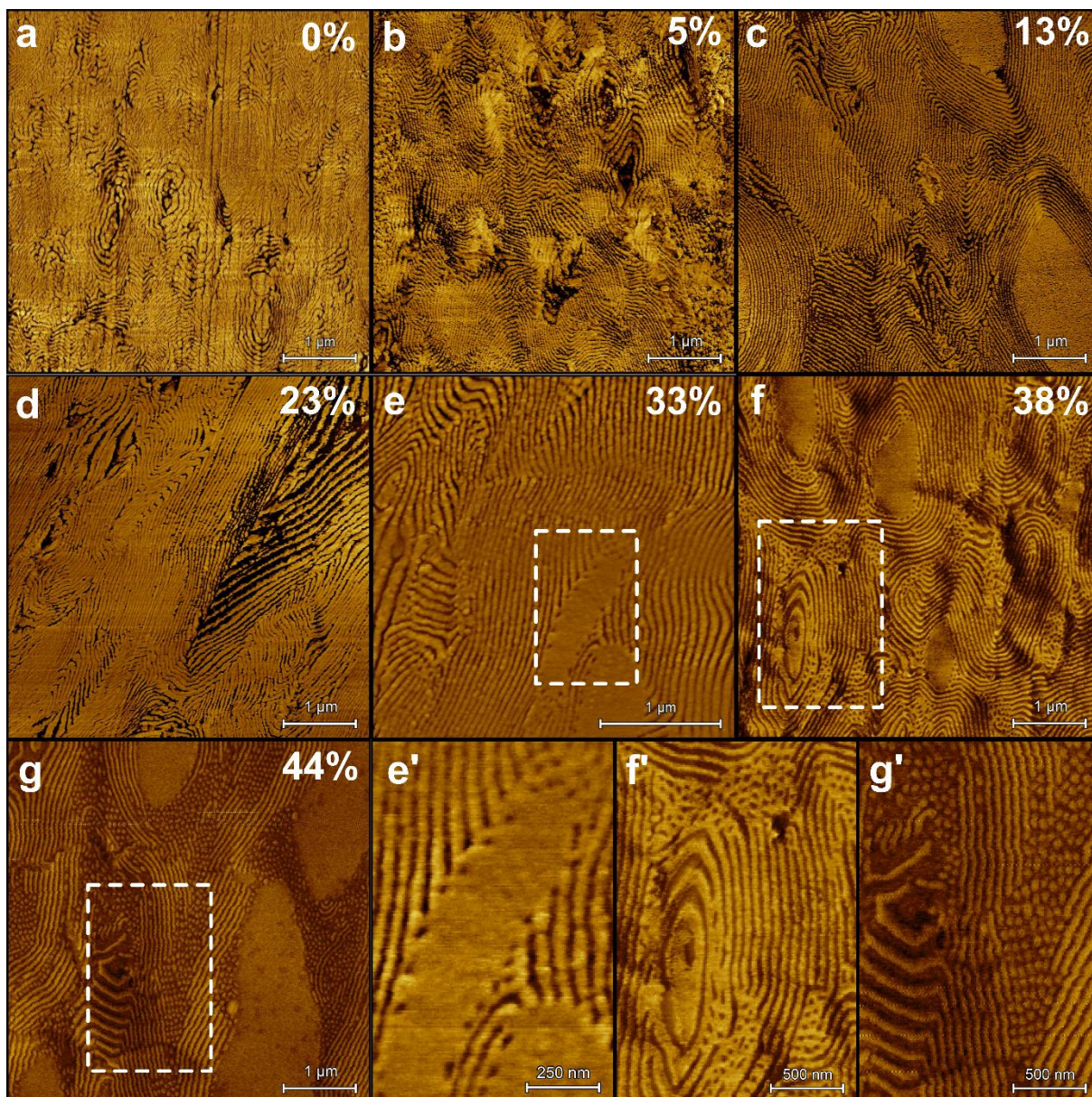
Figure 4. AFM phase images for MAM M52 block copolymer blended with ionic liquids (ILs) over different weight concentrations \phi_{IL} : (a) 0%, (b) 5%, (c) 13%, (d) 23%, (e) 33%, (f) 38%, and (g) 44%. (e'), (f'), and (g') are zoomed images of the squared areas in images (e), (f), and (g), respectively.
