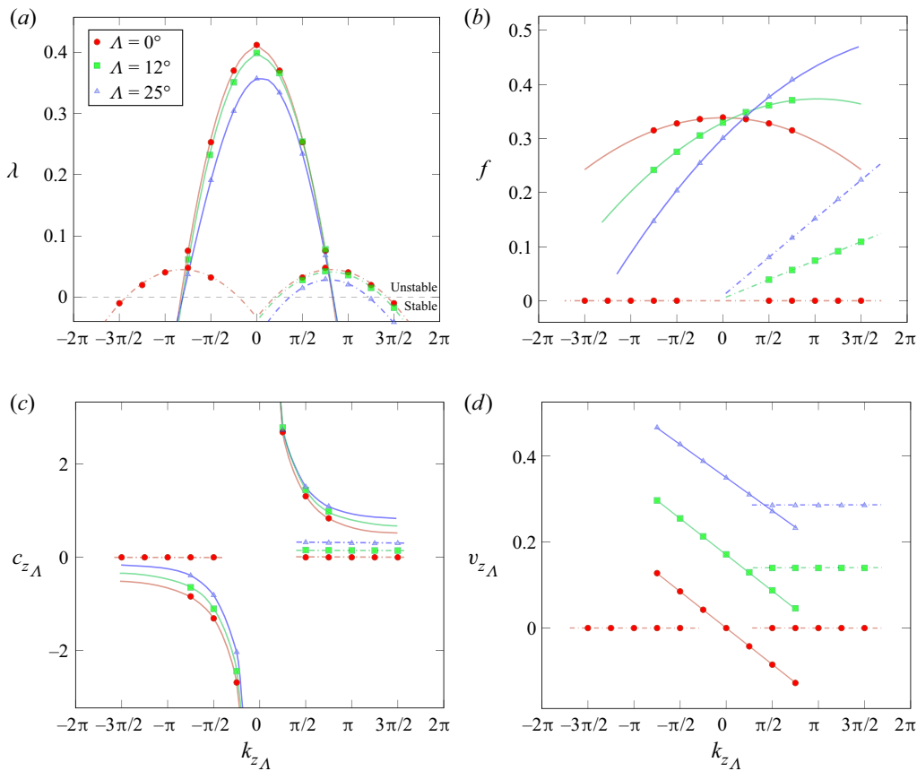
Figure 11. Influence of the sweep angle on the wave properties of the global eigenvalues: (a) growth rate \lambda , (b) frequency f , (c) phase velocity c_{z\Lambda} and (d) group velocity v_{z\Lambda} as functions of the spanwise wavenumber k_{z\Lambda} at \alpha = 20^\circ and Re = 400 for \Lambda = 0^\circ, 12^\circ, 25^\circ .
