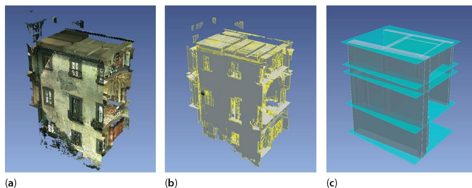
Figure 3. Primitive fitting of perimetral walls and slabs by EdgeWise Building. Raw point cloud (a); fit planes (b); BIM objects (c) using example from Grand-Ducal cloister, Pisa Charterhouse [46].
