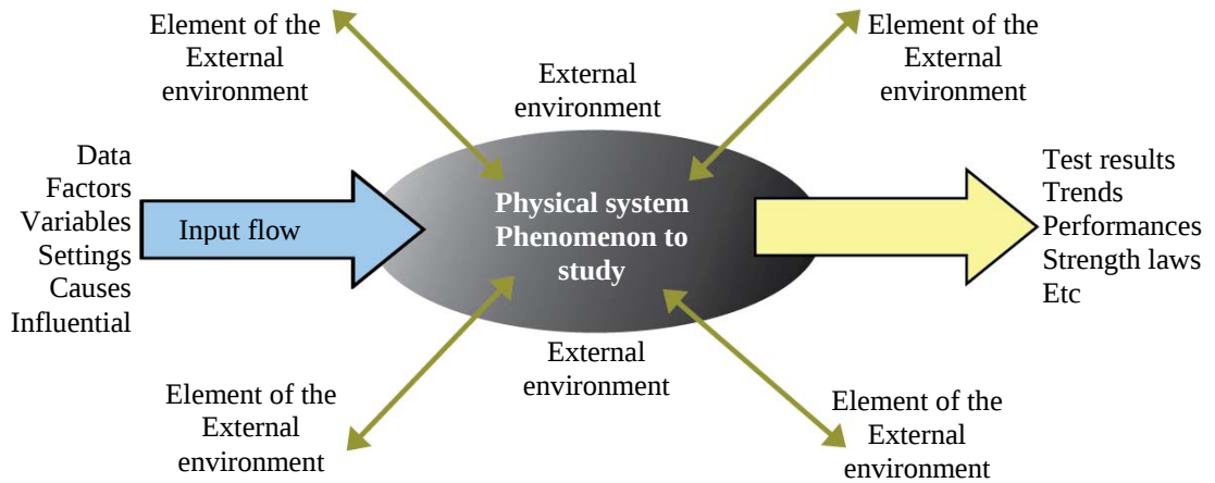
Figure 4: Interactions graph
