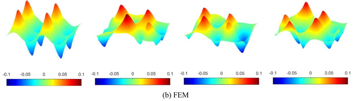
Fig. 17. Comparison of fluctuating temperature distribution \tilde{T} (K) generated by the DHN and FEM reference solution for different microstructures.
