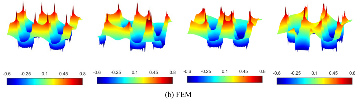
Fig. 18. Comparison of fluctuating temperature gradient \tilde{H}_2 (K/m) distribution generated by the DHN and FEM reference solution for uniform fiber arrangement.
