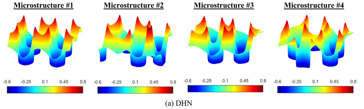
Fig. 17. Comparison of fluctuating temperature distribution \tilde{T} (K) generated by the DHN and FEM reference solution for different microstructures.
